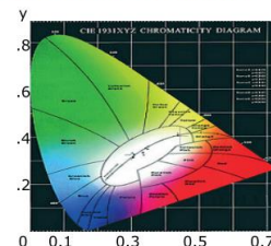
E1931 CHROMATICITY DIAGRAM
