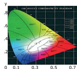
:1931 CHROMATICITY DIAGRAM
