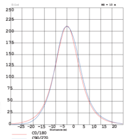
Planar Illuminance Curve
